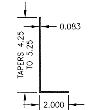
TRACK ANGLE
