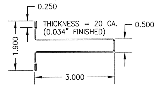
3" REINFORCING STRUT
