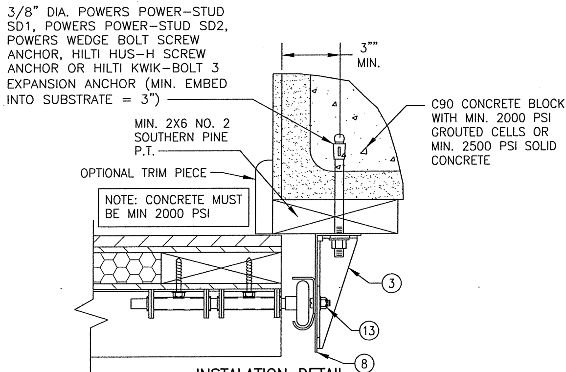
INSTALLATION DETAIL SHIMMED TO FILLED BLOCK OR SOLID CONCRETE
