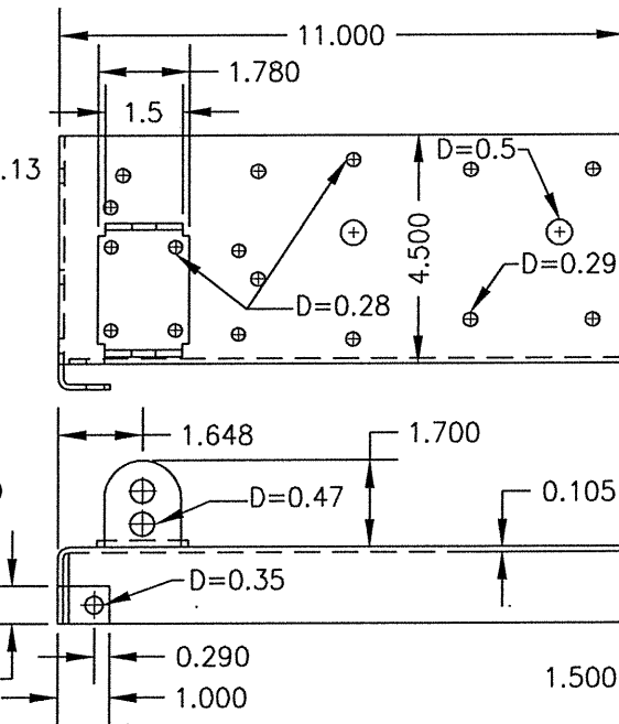
BOTTOM CABLE BRACKET
