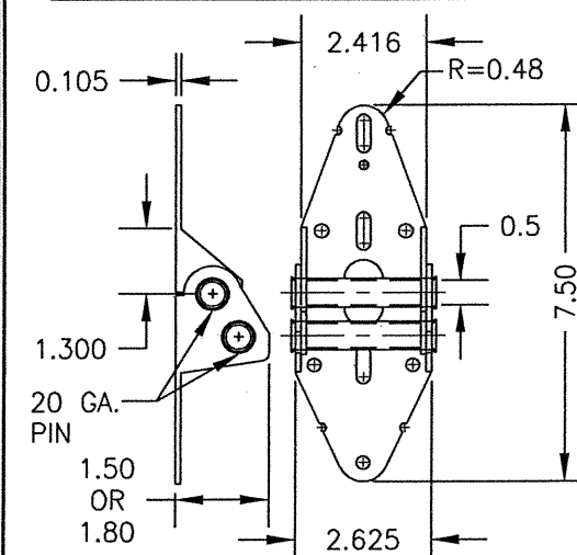
DOUBLE PIN HINGE
