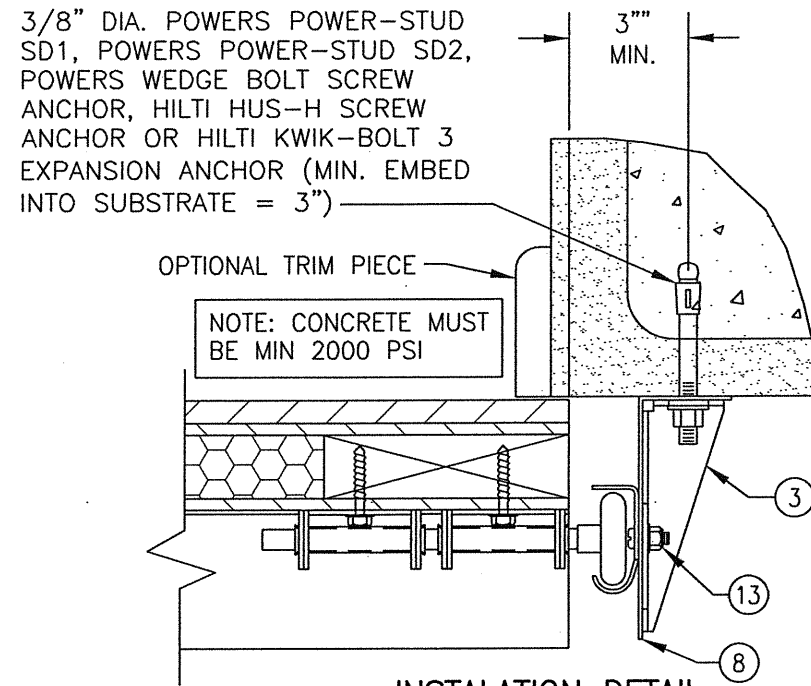
INSTALLATION DETAIL DIRECT TO FILLED BLOCK OR SOLID CONCRETE
