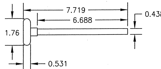
NYLON ROLLER WITH AISI STEEL ROD
